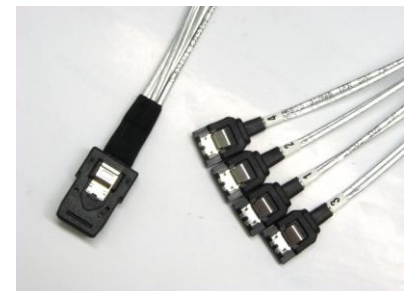
AMPH-874S-XXX: SFF-8087 to 4 SATA2 Cable with XXX as the standard or customized length in cm
